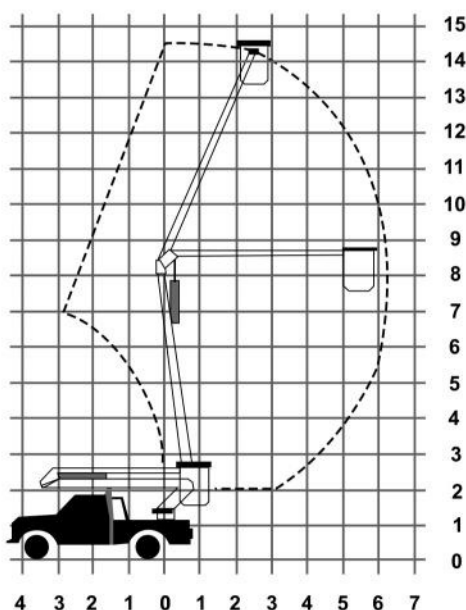
Diagrama de Alcances VAM 200/15 - 200/15 A
